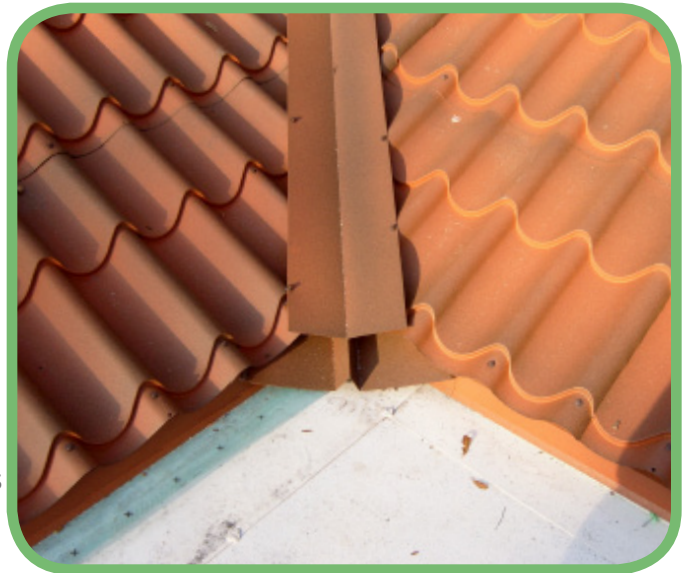
Exposed Through-Fastened Tile profile Steel Roof
